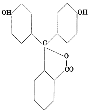
Phenolphthalein.
